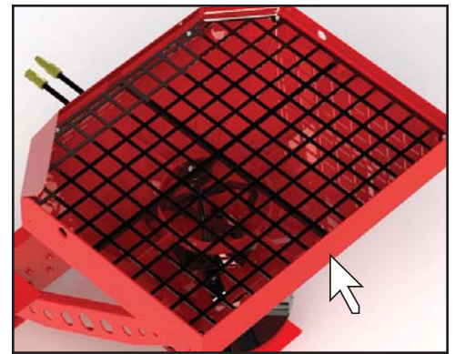
Self-loading Hopper with Cutting Edge and Protective Grate.
