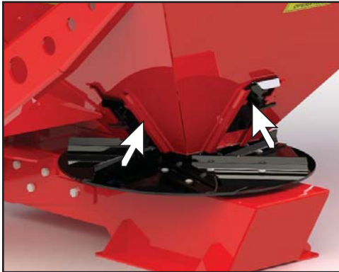
Adjustable Gates to control material flow.
